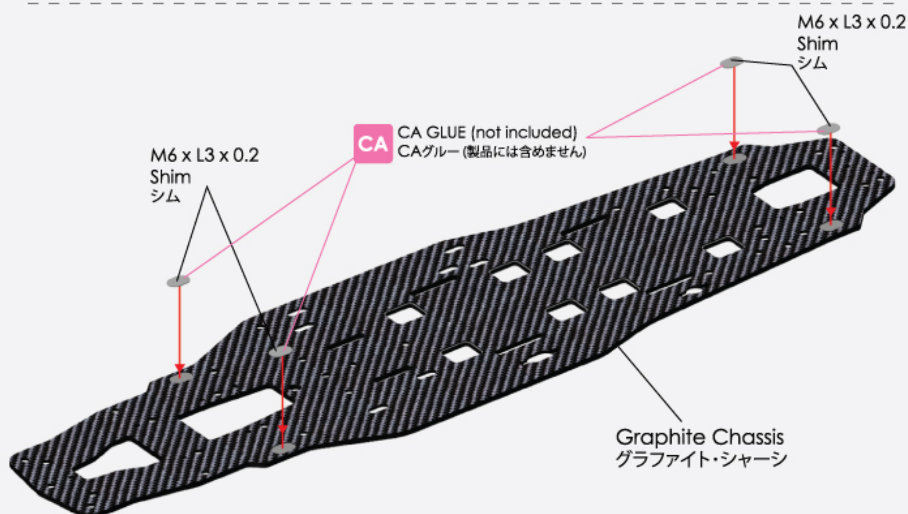
assemble view 組立図
